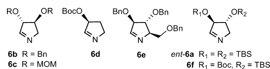
Figure 2. Optically active five-membered cyclic imines.
