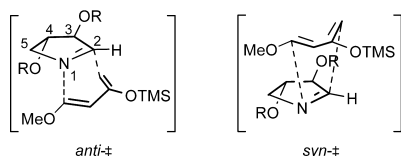
Figure 3. Diastereoselectivity of the cycloaddition.
